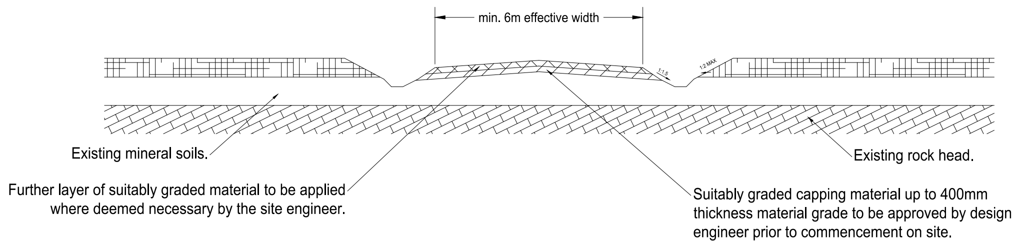
TYPICAL TRACK FORMATION ON OVERBURDEN SOIL SCALE 1:100
