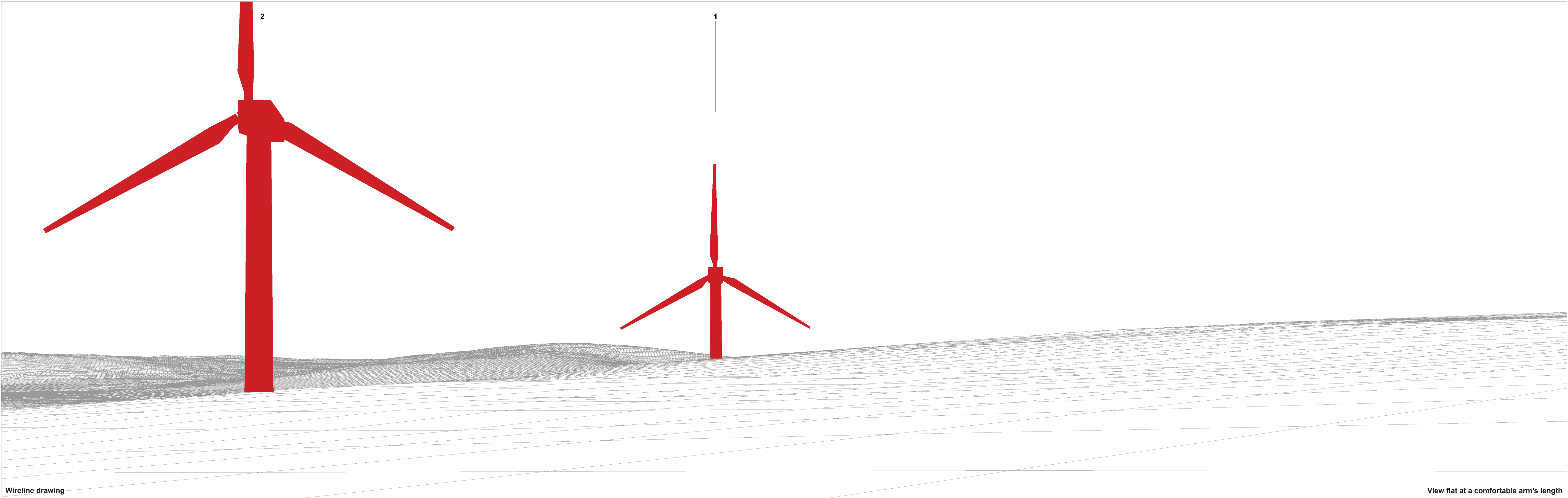
Figure: 6.4.1a RVAA Viewpoint 1: Veltan Nisthill Wind Farm
